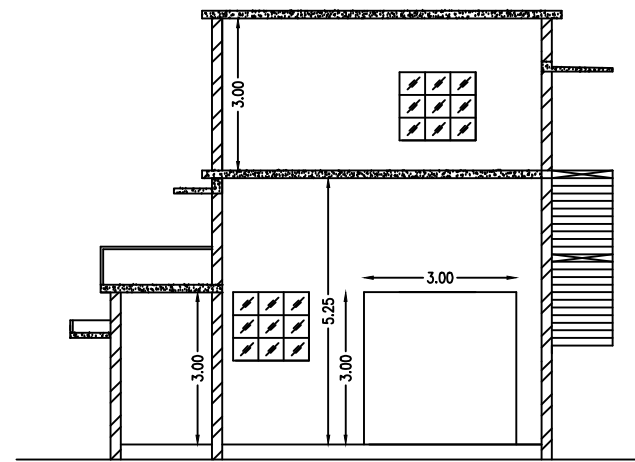
SECTION YY
