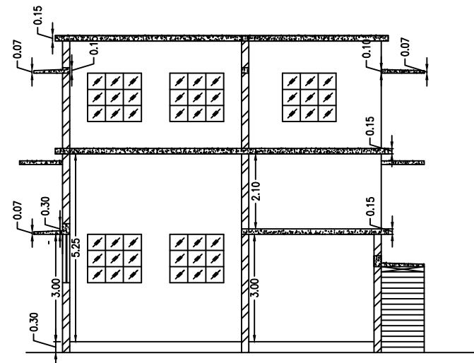
SECTION XX
